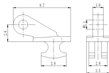
塑铰 Regular hinge for plastic hinge
