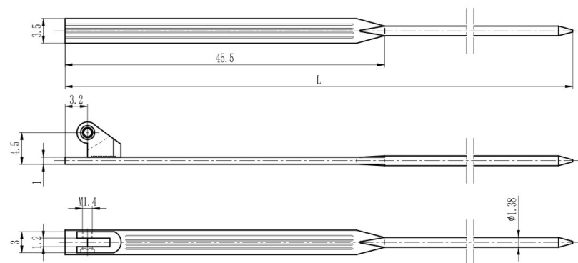
铰链插芯 Regular hinge wire core L136 XHD4193-1360-YN 材料/Material: 无铅白铜/Lead free nickel silver
