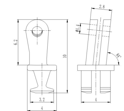
塑铰 Regular hinge for plastic frame XA3069B50/WG01
