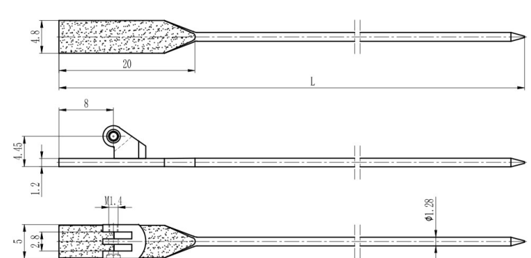
铰链插芯 Regular hinge wire core
