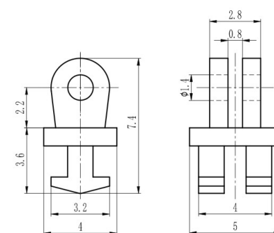
塑铰 Regular hinge for plastic frame
