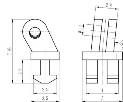
塑铰 Regular hinge for plastic frame XA005B50/WG01
