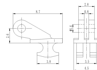
塑铰 Regular hinge for plastic frame XA071-D45/N0
