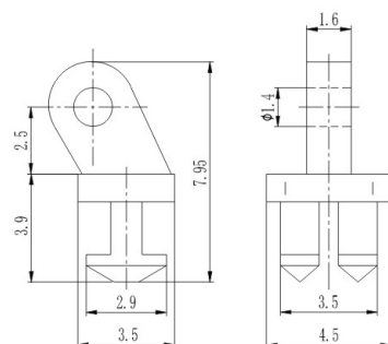
塑铰 Regular hinge for plastic hinge
