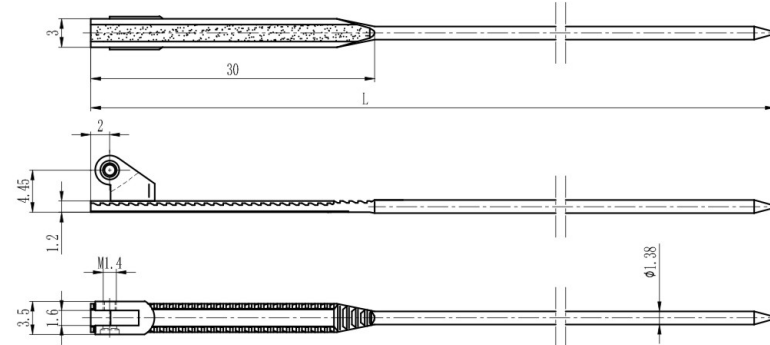
铰链插芯 Regular hinge wire core L125 XHP2165G1250/YG01 L130 XHP2165G1300/YG01 材料/Material: 无铅白铜/Lead free nickel silver
