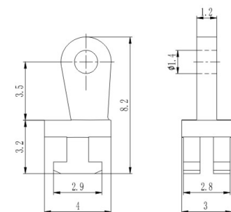
塑铰 Regular hinge for plastic frame XAA383-30-WN 材料/Material: 无铅白铜/Lead free nickel silver
