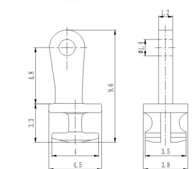
塑铰 Regular hinge for plastic frame XAA3169H38-WN 材料/Material: 无铅白铜/Lead free nickel silver
