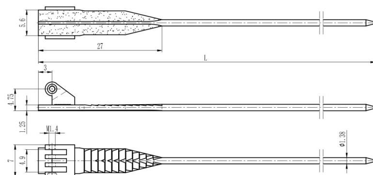
对口铰 Regular hinge for metal frame XB170-A70/W 材料/Material: 无铅白铜/Lead free nickel silver
