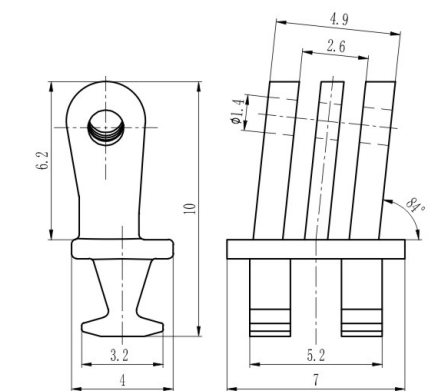
塑铰 Regular hinge for plastic frame XA3069-70/WG01 材料/Material: 无铅白铜/Lead free nickel silver
