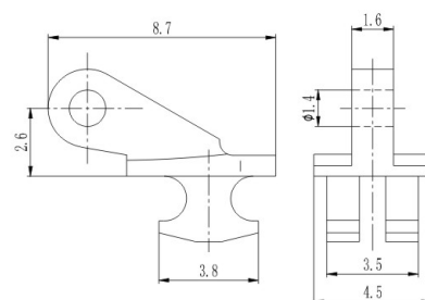
塑铰 Regular hinge for plastic hinge XA071-45/NO
