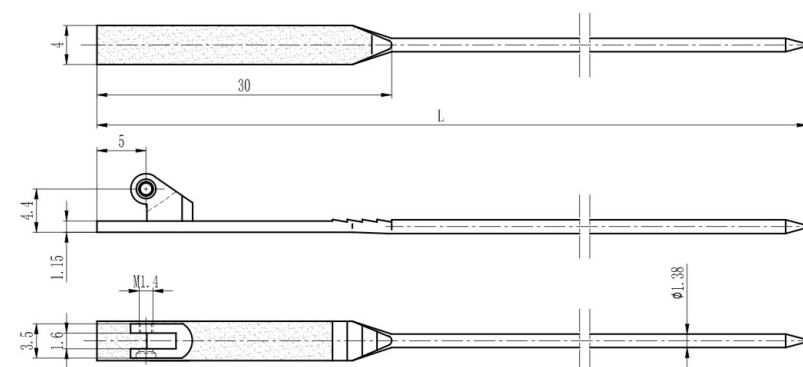
铰链插芯 Regular hinge wire core L130 XHP1650-H1300/YG01 L135 XHP1650-H1350/YG01 材料/Material: 无铅白铜/Lead free nickel silver
