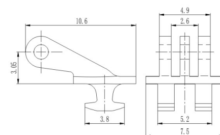
塑铰 Regular hinge for plastic frame XAA4121-75-WN 材料/Material: 无铅白铜/Lead free nickel silver
