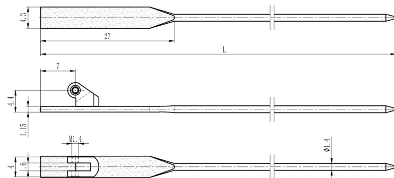
铰链插芯 Regular hinge wire core
