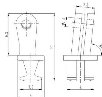
塑铰 Regular hinge for plastic frame
