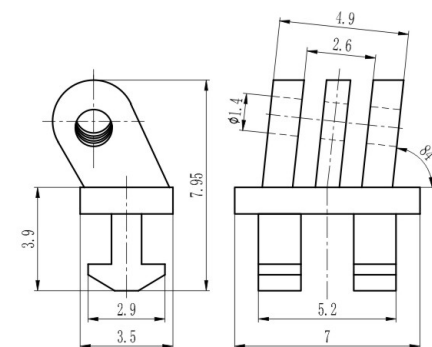
塑铰 Regular hinge for plastic frame XA005-N70/N0 材料/Material: 无铅白铜/Lead free nickel silver
