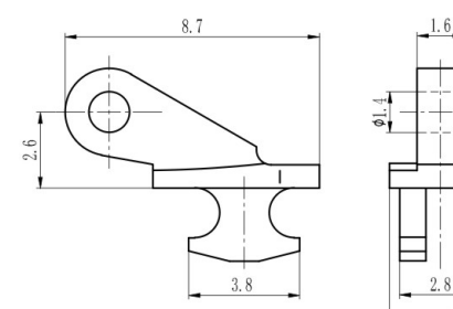
塑铰 Regular hinge for plastic frame XA071-35/N0 材料/Material: 无铅白铜/Lead free nickel silver
