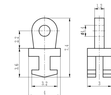
塑铰 Regular hinge for plastic frame XA119C30/N0 材料/Material: 无铅白铜/Lead free nickel silver
