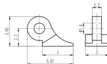
对口铰 Regular hinge for metal frame XB007-30/W 材料/Material: 无铅白铜/Lead free nickel silver
