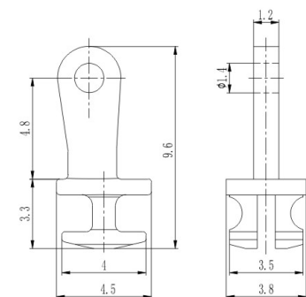
塑铰 Regular hinge for plastic frame XAA3169H38-WN 材料/Material: 无铅白铜/Lead free nickel silver
