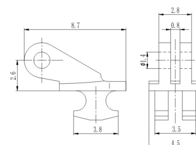
塑铰 Regular hinge for plastic frame
