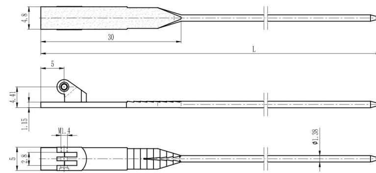
铰链插芯 Regular hinge wire core
