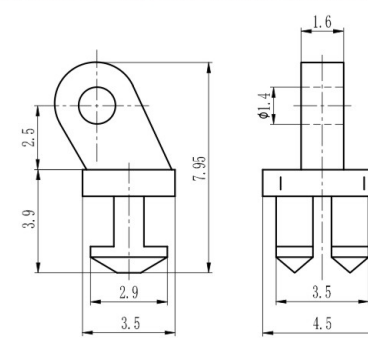
塑铰 Regular hinge for plastic frame XA005F45/N0 材料/Material: 无铅白铜/Lead free nickel silver
