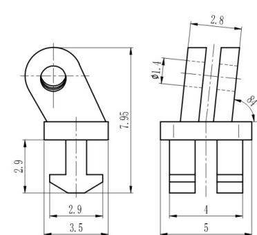
塑铰 Regular hinge for plastic frame
