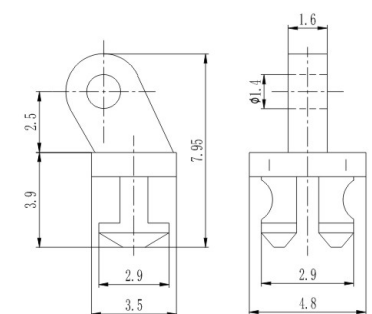
塑铰 Regular hinge for plastic hinge XA005A48/N0
