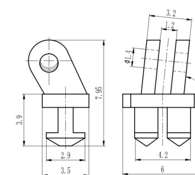
塑铰 Regular hinge for plastic frame
