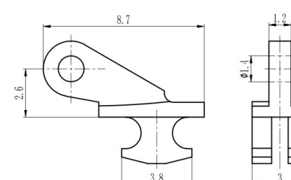
塑铰 Regular hinge for plastic frame XA071-A30/WG01 材料/Material: 无铅白铜/Lead free nickel silver
