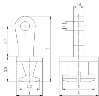
塑铰 Regular hinge for plastic hinge
