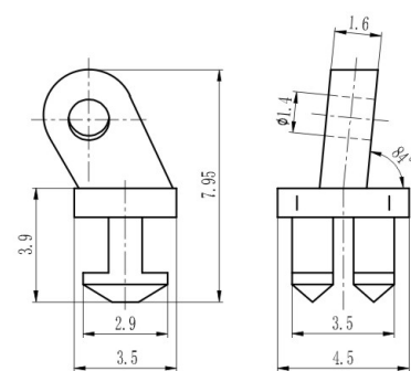
塑铰 Regular hinge for plastic hinge XA005A45/N0
