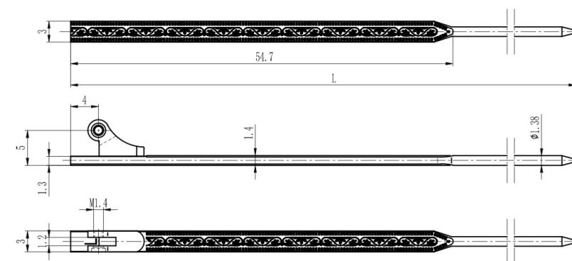
铰链插芯 Regular hinge wire core L139 XHD2361EA1390-YN 材料/Material: 无铅白铜/Lead free nickel silver
