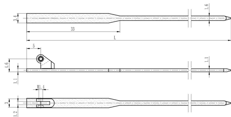
铰链插芯 Regular hinge wire core L136 XHD2080CA1360-YN 材料/Material: 无铅白铜/Lead free nickel silver
