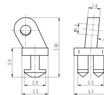
塑铰 Regular hinge for plastic frame XA005A45/N0 材料/Material: 无铅白铜/Lead free nickel silver
