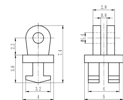
塑铰 Regular hinge for plastic frame XA119D50/N0
