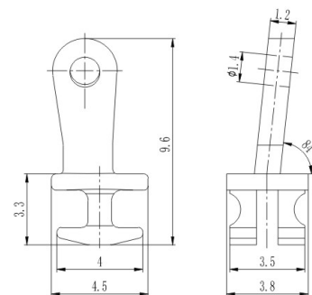
塑铰 Regular hinge for plastic frame XAA3169E38-WN 材料/Material: 无铅白铜/Lead free nickel silver
