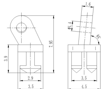
塑铰 Regular hinge for plastic hinge XA005A45/N0
