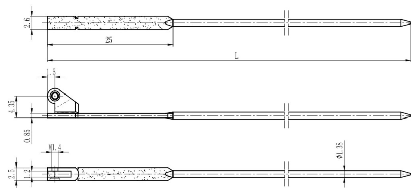
铰链插芯 Regular hinge wire core L130 XHP1200C1300/YG01 L135 XHP1200C1350/YG01 材料/Material: 无铅白铜/Lead free nickel silver
