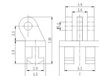
塑铰 Regular hinge for plastic frame XA005-M70/N0 材料/Material: 无铅白铜/Lead free nickel silver
