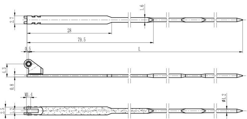
铰链插芯 Regular hinge wire core L130 CHD2226K1300-YN 材料/Material: 不锈钢/Stainless steel
