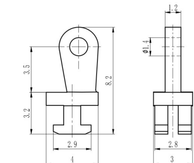
塑铰 Regular hinge for plastic frame XAA383-30-WN 材料/Material: 无铅白铜/Lead free nickel silver
